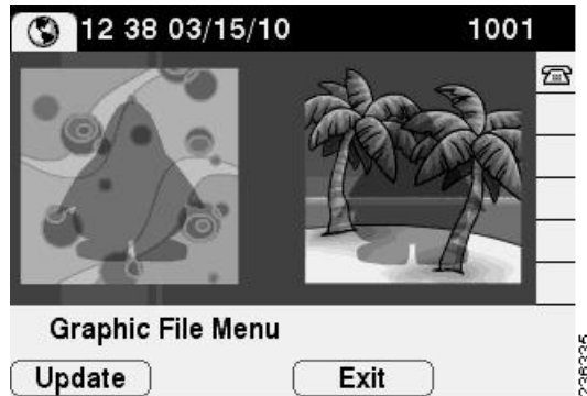
Figure 3-8 CiscoIPPhoneGraphicFileMenu
