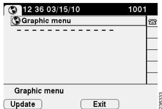
Figure 3-6 CiscoIPPhoneGraphicMenu Object
