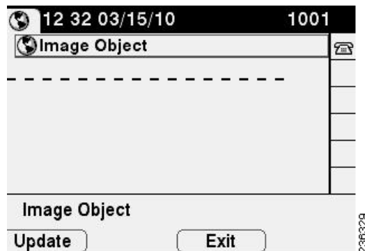
Figure 3-4 CiscoIPPhoneImage Object
